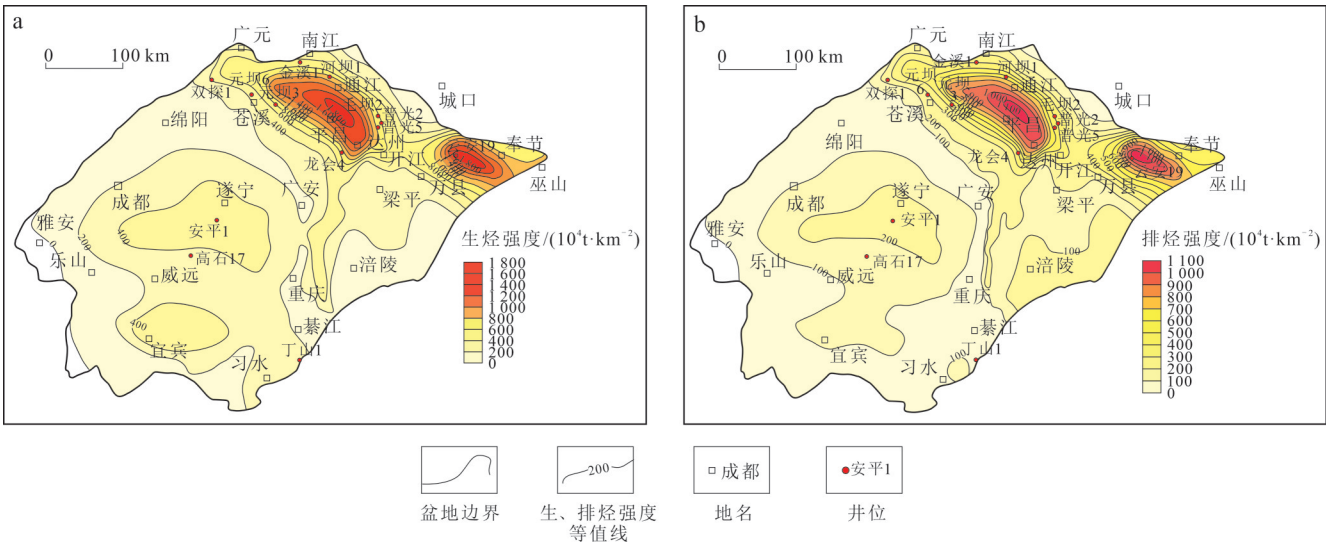
图9 现今四川盆地上二叠统龙潭组烃源岩生、排烃强度 Fig. 9 Hydrocarbon generation and expulsion intensity of the source rocks from the Longtan Formation in the Upper Permian of the Sichuan Basin at present a. 生烃强度; b. 排烃强度
