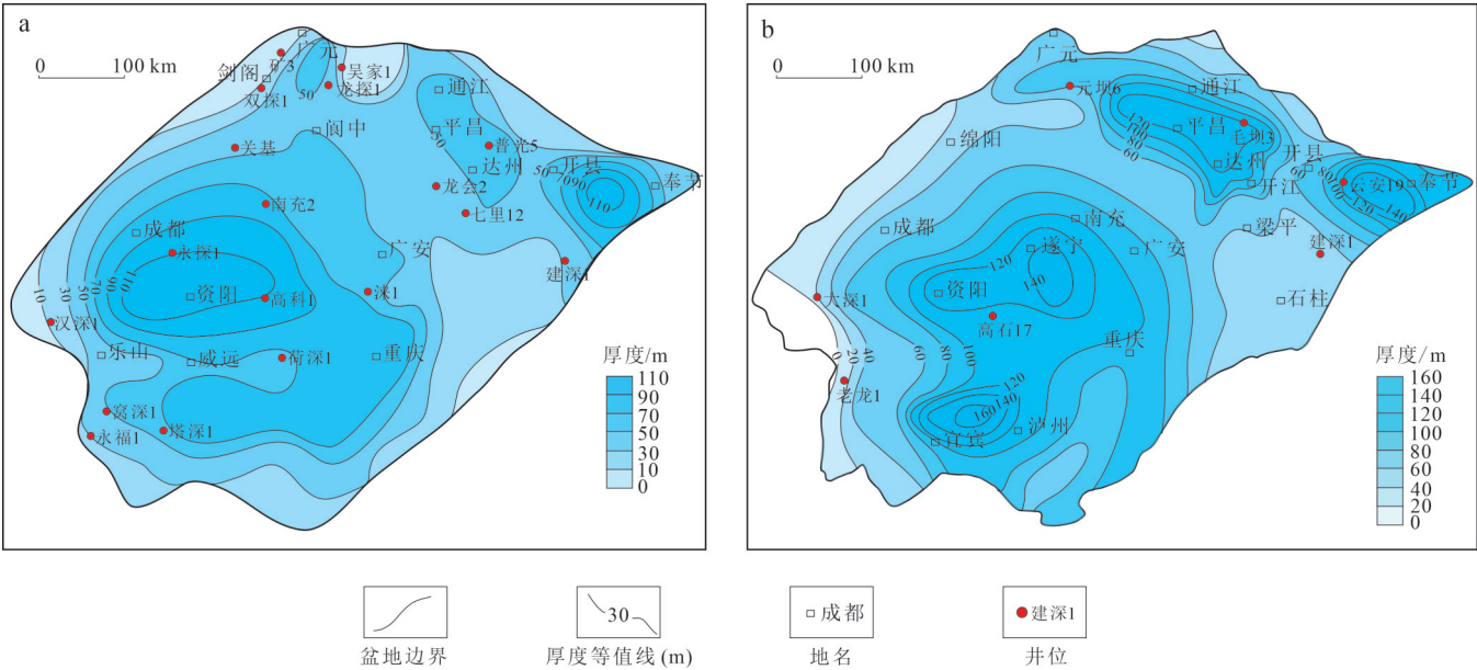
图10 第四次资源评价所用的上二叠统泥质烃源岩厚度(a)与上二叠统龙潭组烃源岩厚度(b) Fig. 10 Isopach maps of argillaceous source rocks used for the Fourth Resource Evaluation (a) and of source rocks of Longtan Formation of Upper Permian (b)
